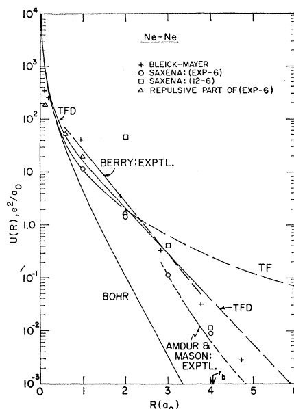
FIG. 6. Repulsive interaction potentials for the Ne-Ne system.
