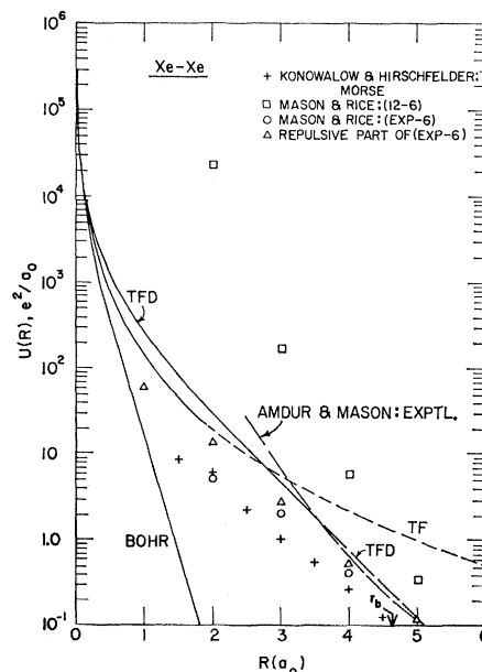
FIG. 10. Repulsive interaction potentials for the Xe-Xe system.
